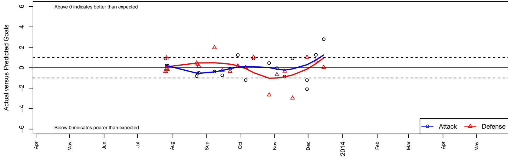
NSC Revolution B95 Dots are actual minus expected GF (blue circles) and GA (red triangles). Blue line is smoothed change in attack strength. Red is smoothed change in defense strength.
